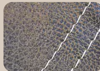
Contrasterend stiksel
